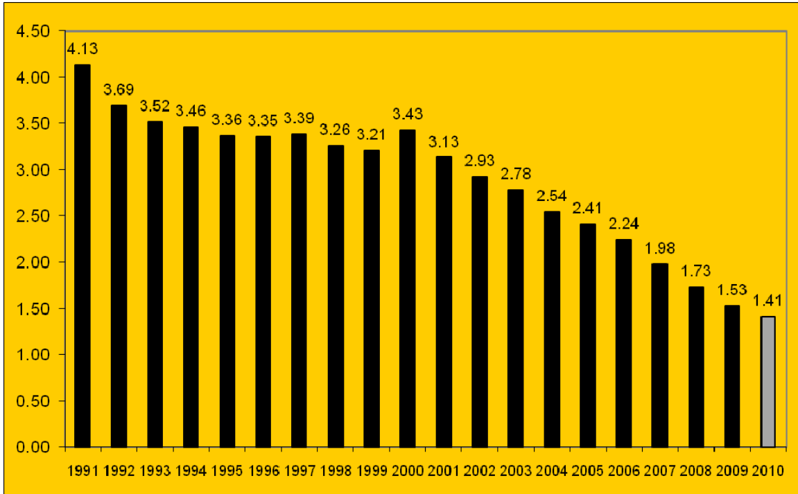
Figure 1: The lost-time claim rate*, Alberta 1991 to 2010
